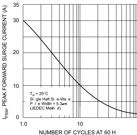
Fig. 3 Maximum Peak Forward Surge Current (typical)
