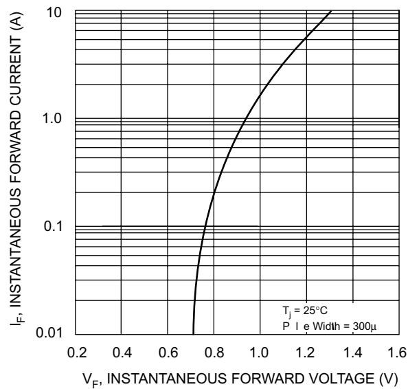
Fig. 2 Typical Forward Characteristic (typical)
